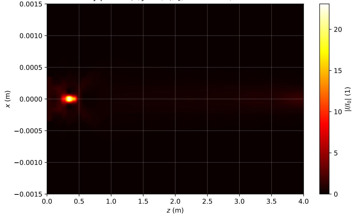
Intensity profile I(x, y = 0, z)/I_0 , P_{in}=3.0P_{cr} , artificial time
